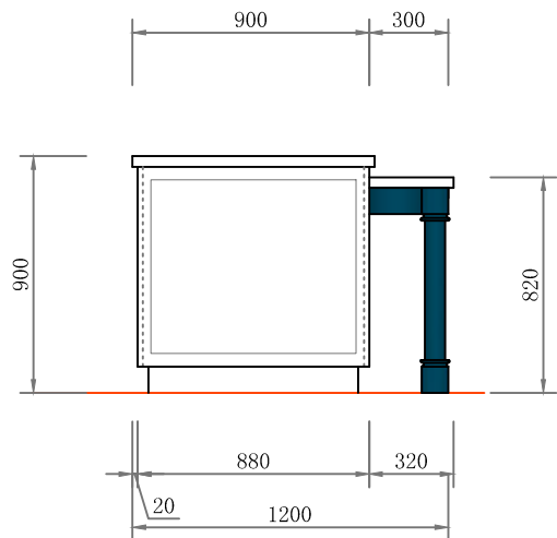
ELEVATION F
