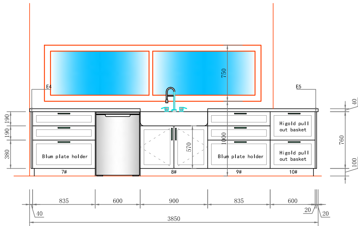
ELEVATION C
