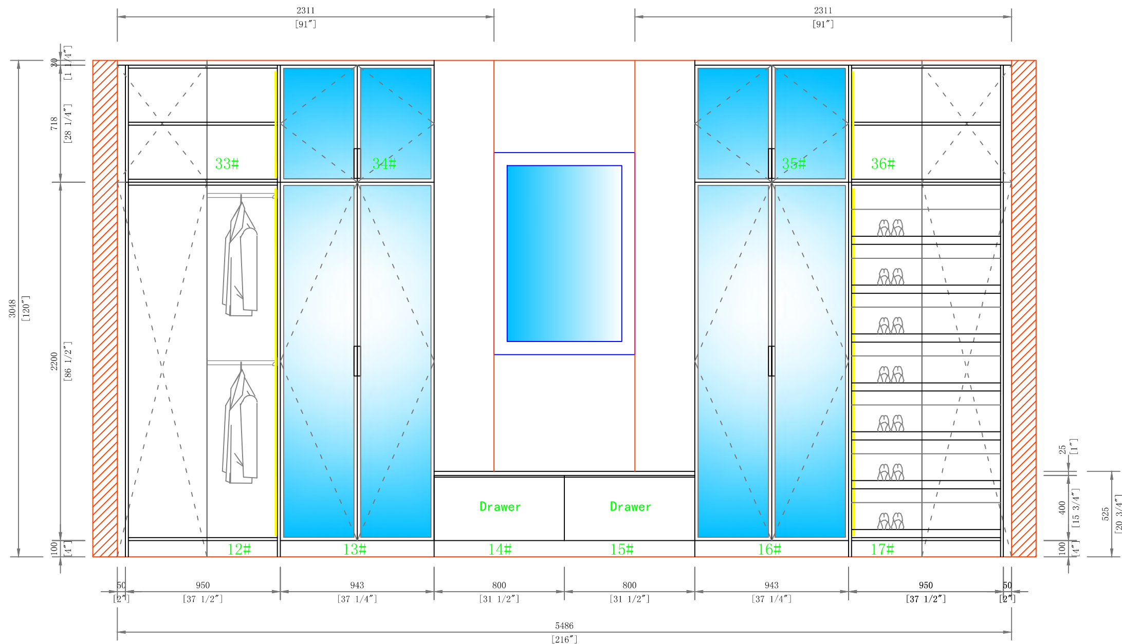
ELEVATION D
