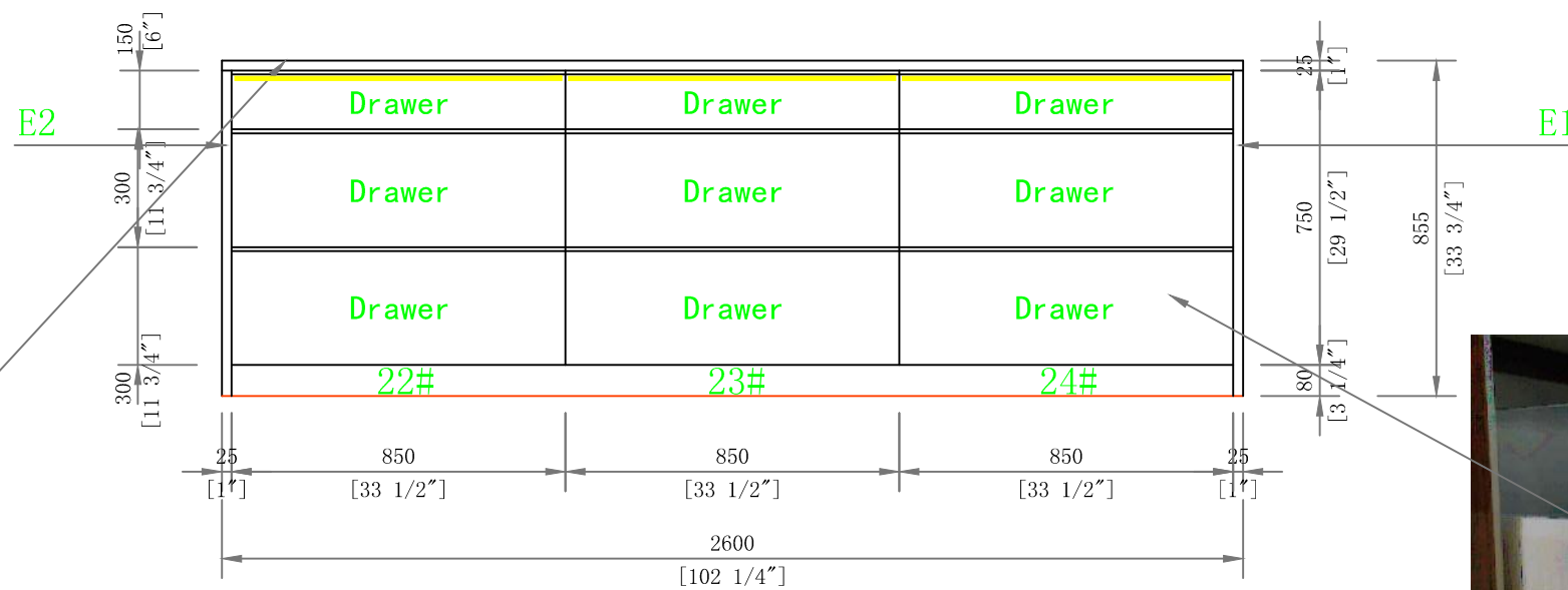
ELEVATION F
