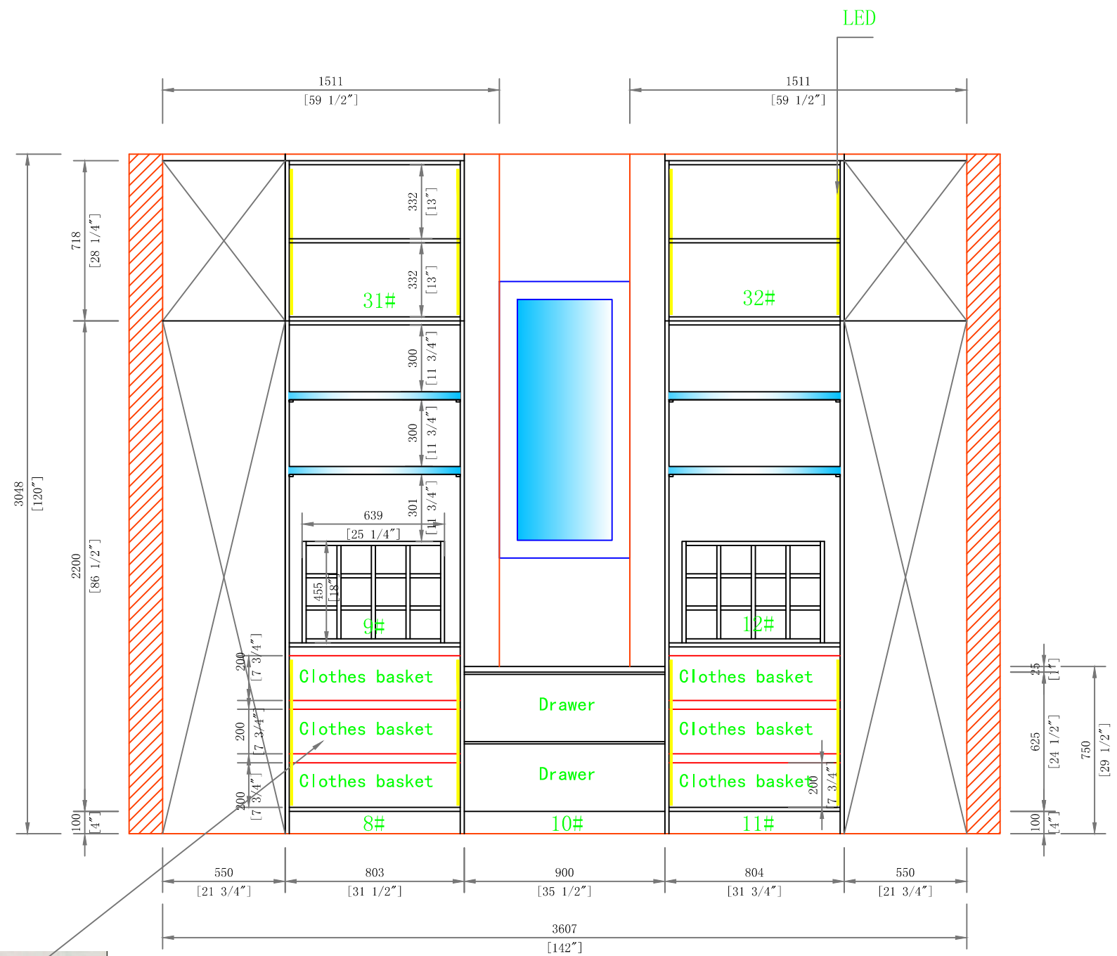
ELEVATION C
